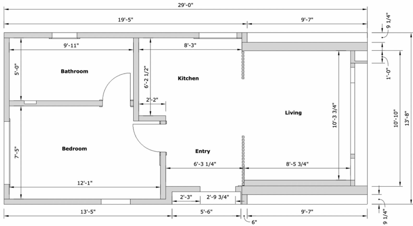
Wall Plan
